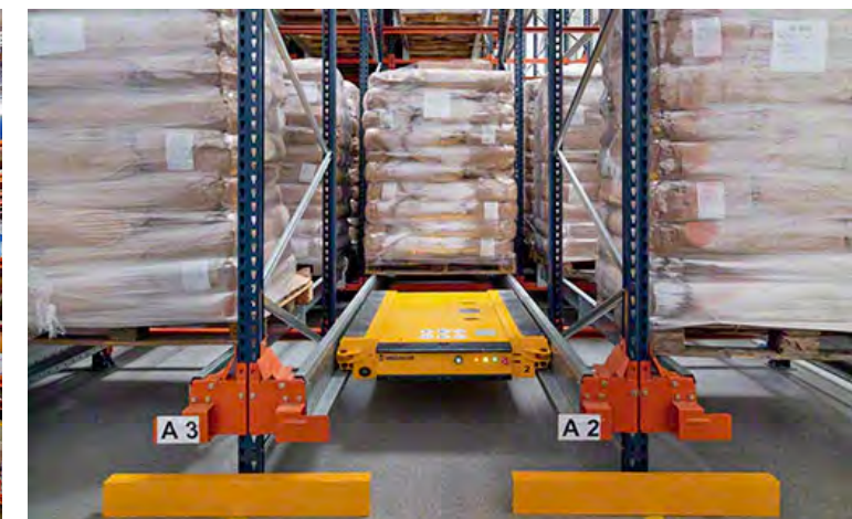
Pallet Shuttle Semi-automatic electric shuttle loads and unloads pallets inside compact racks.
