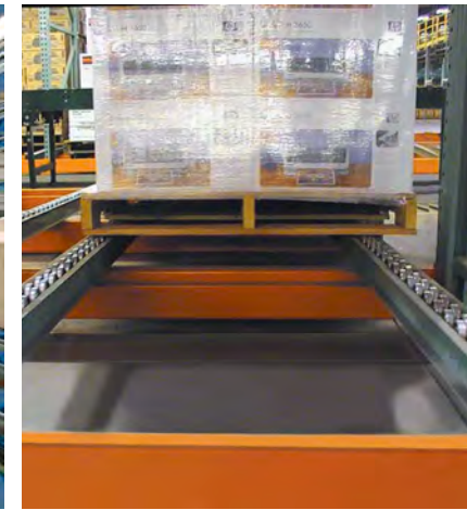
Pallet Flow Racks - FIFO Precise pallet rotation.
